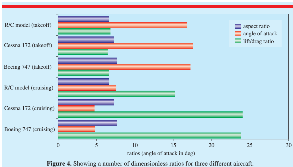
Figure 4. Showing a number of dimensionless ratios for three different aircraft.
